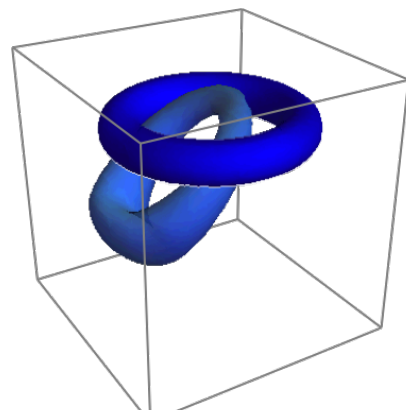
Wavefunction of the Schrödinger cat state of the Rydberg atom. The electron is in a quantum superposition of two classical trajectories (dark blue and light blue) with very different electric dipoles, making the state highly sensitive to the electric field.
